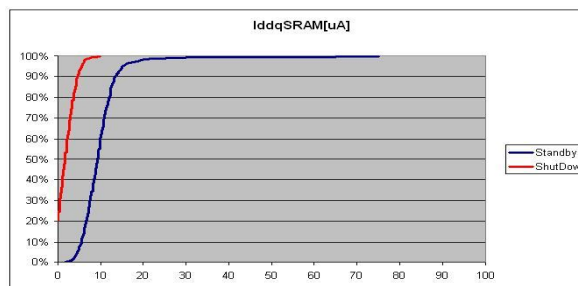
Figure 4: Plot of VDDram IDDQ
