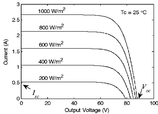
Fig. 4. I-V characteristic curves of the PV model at different irradiances.
