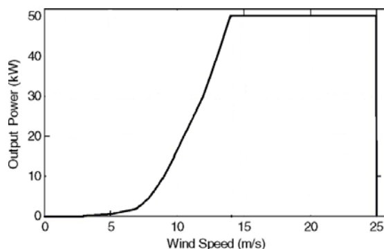
Fig. 3. Wind turbine output power characteristic curve
