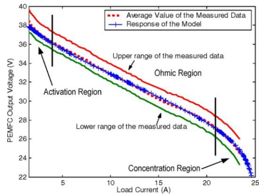
Fig. 6. PEMFC V-I characteristic: comparison of model response with experimental data
