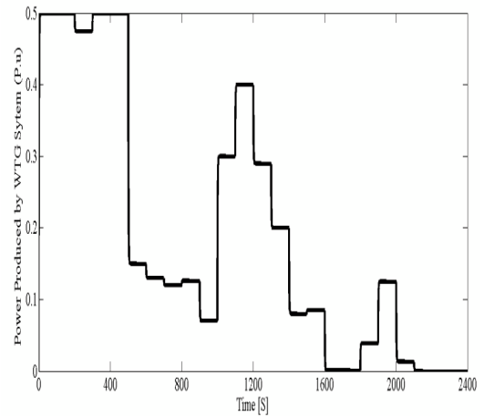
Fig. 7. Power produced by wind turbine generator
