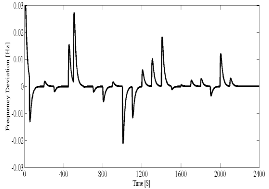
Fig. 12. Frequency deviation
