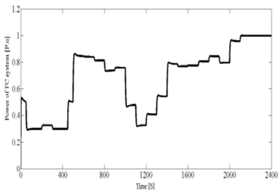
Fig. 11. Power supplied by the FC stack for whole day
