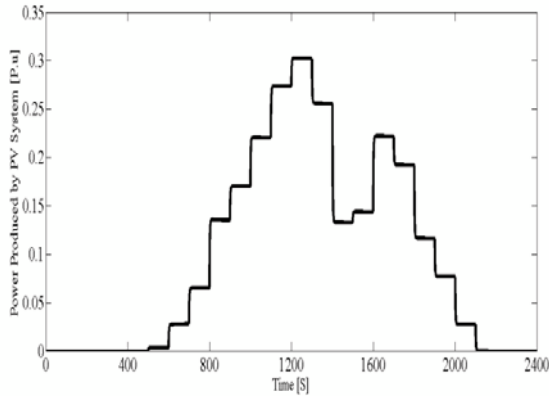
Fig. 8. PV power generated for whole day
