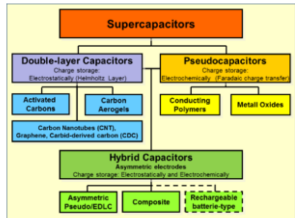
Fig 7 : Hierarchical classification of supercapacitors and related types
