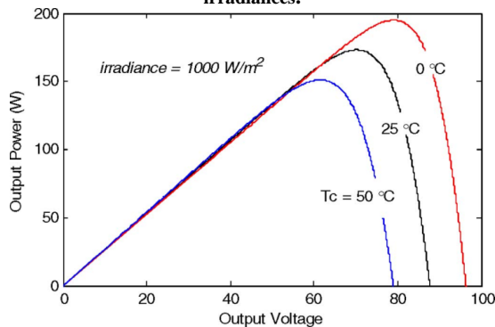
Fig. 5. P-V characteristic curves of the PV model at different operating temperatures
