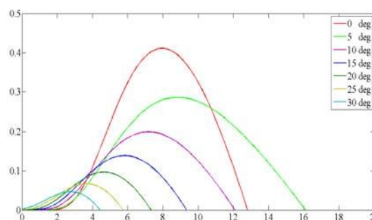
Fig. 2. C_p - \lambda characteristics of the wind turbine generator at different pitch angles ( \theta ).
