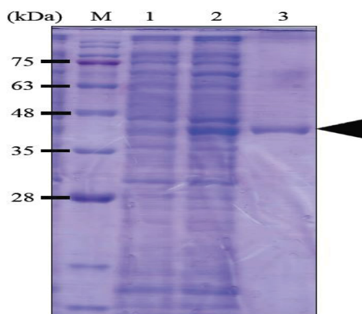
Figure 4. Purification of recombinant CpurFLS2 . Lane M: Protein Marker; Lane 1: E. coli Lysate without IPTG; Lane 2: E. coli Lysate with 10 μM IPTG; Lane 3: The Purified Recombinant Protein. The purified CpurFLS2 recombinant protein is indicated by an arrowhead.
