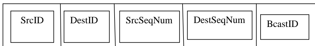
Fig. 3 Format of route request in AODV
