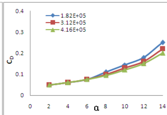
Fig 8- Variation of Drag coefficient with angle of attack
