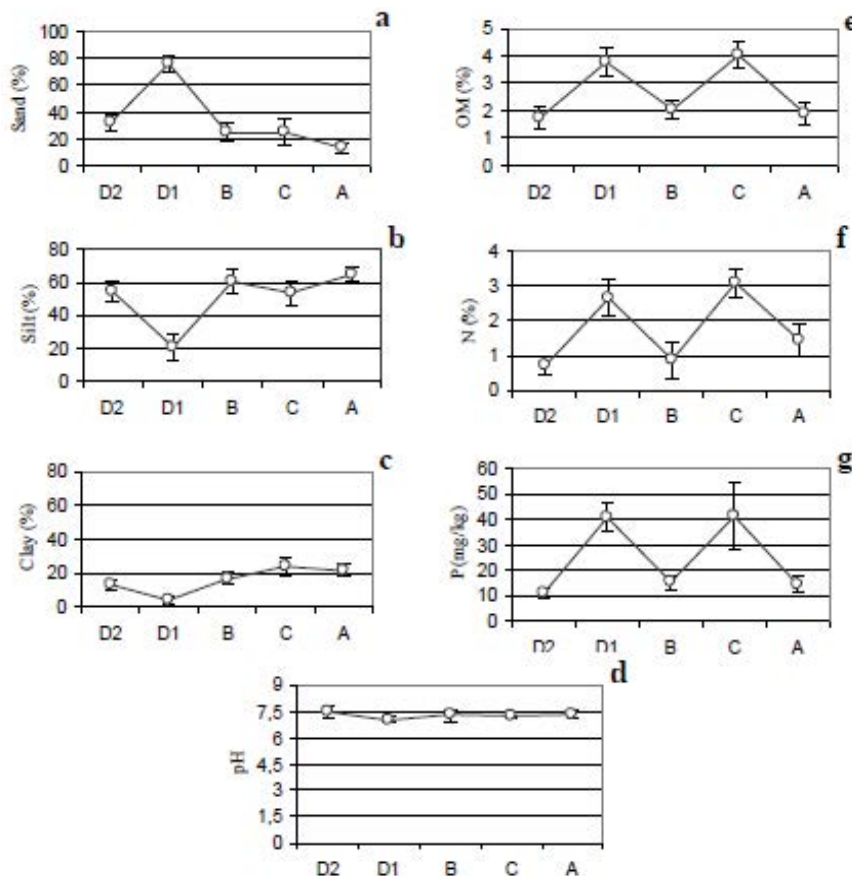
Figure 3. contents of sand (3a), silt (3b), clay (3c), concentrations of organic matter (OM) (3e), nitrogen (N) (3f), phosphorus (P) (3g) and pH values in the different sites (A=Mountain, B=Glacis, C=Wadis, D1=Sandy plain, D2=Silty plain).
