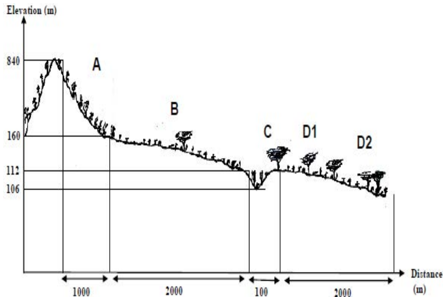
Figure 2. Geomorphological schema of the study area. A=Mountain, B=Glacis, C=Wadis, D1=Sandy plain, D2=Silty plain.
