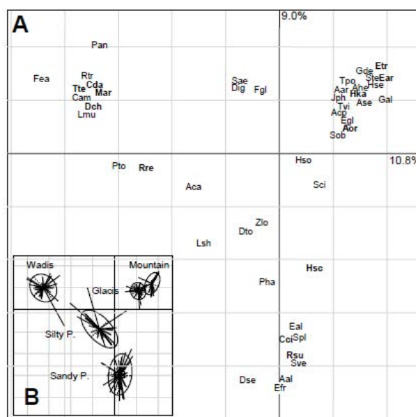
Figure 4. Correspondence analysis of presence-absence data (200 relevés and 47 species). A: Axis 1 (horizontal) and 2 (vertical) representation of vegetation species (most contributive species in bold). B: Axis 1 and 2 representation of relevés. Relevés are categorised according to 4 landform types : Wadis, Plain (sandy or silty), Glacis and Mountain. Landform types are represented as inertia ellipses. Mean and individual situation of the relevés per each landform type are represented by stars.
