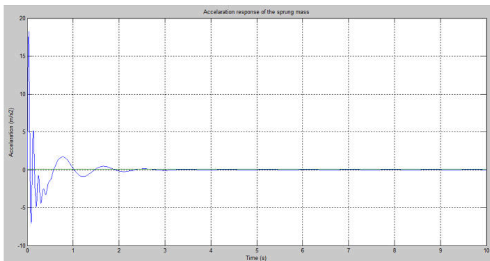
Fig. 8 Step input and Acceleration response of sprung mass
