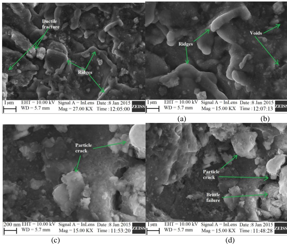
Fig. 7 Tensile fractured surface SEM image of (a) AA6063 with 5% Cenosphere (b) AA6063 with 10% Cenosphere (c) AA6063 with 15% Cenosphere (d) AA6063 with 20% Cenosphere
