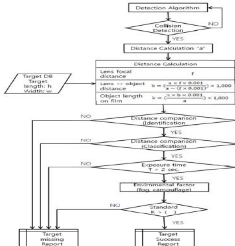
Figure 4: The target detection algorithm of the usam.
