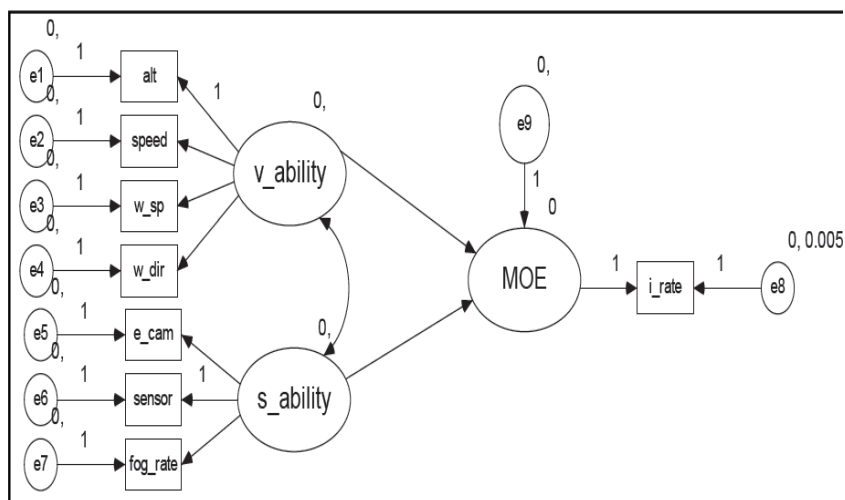
Figure 6: The observed model for structural equation modeling.
