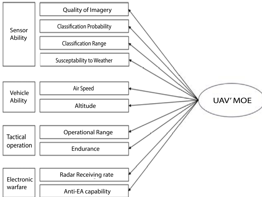
Figure 3: The model resulted by factor analysis.
