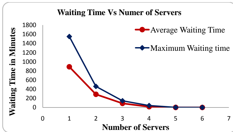
Fig. 5 Simulation Result of Waiting Time Vs Number of Servers
