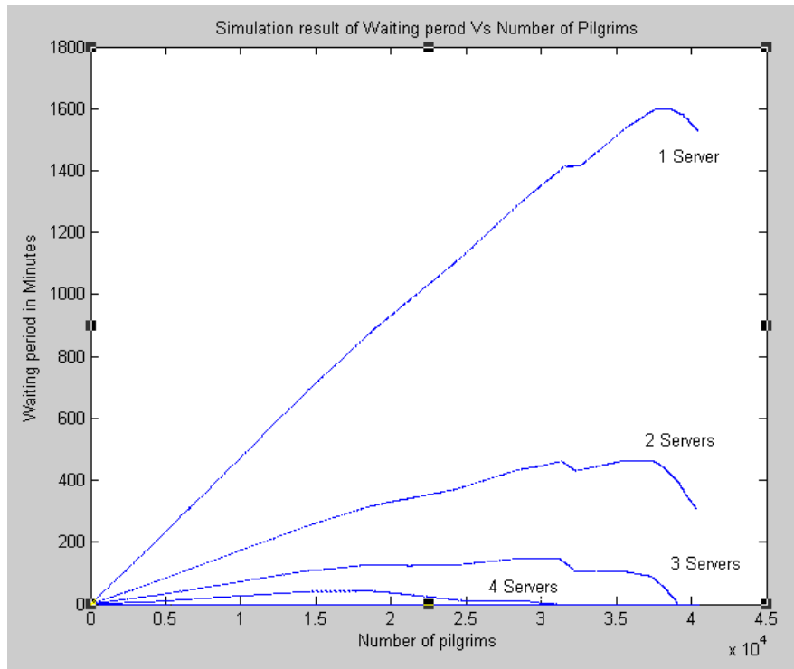
Fig. 6 Simulation of Individual Waiting Time of each Pilgrims Vs Number of Servers by Matlab
