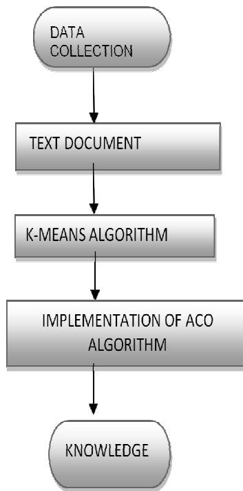
Fig.3. Clustering Process
