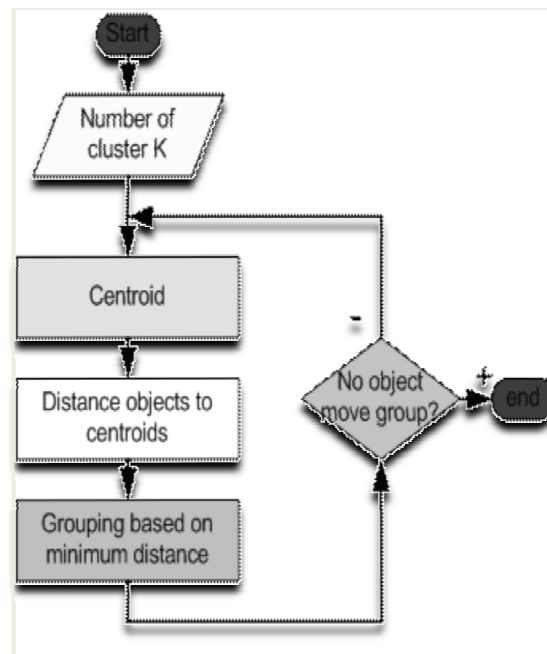
Fig.2. K-Means process
