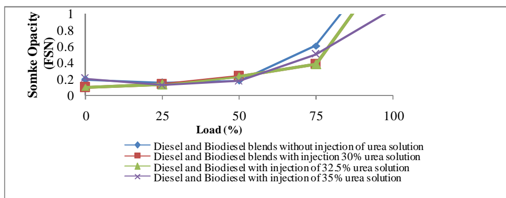
Fig. 3.8 Variation of Smoke Opacity with engine load for varying urea concentration (Biodiesel)
