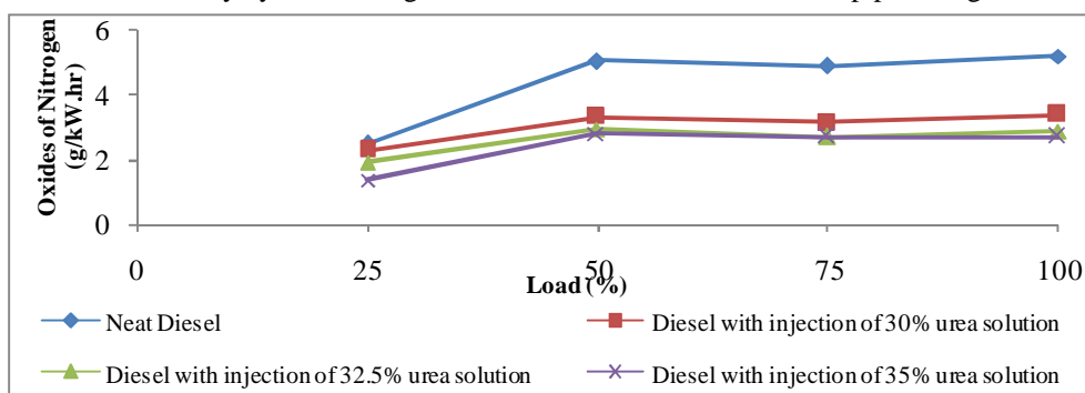
Fig.3.1 Variation on oxides of Nitrogen with Engine Load (Varying urea concentration)
