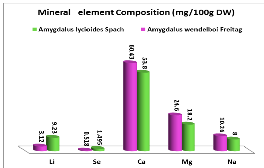
Figure 2- The Mean content (mg/100g DW) of Na, Mg, Ca, Se and Li composition in A. lycioides and A. wendelboi kernel samples.
