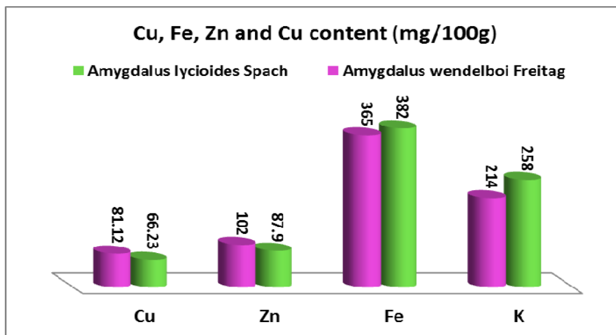
Figure 3- The Mean content (mg/100g DW) of K, Zn and Cu composition in A. lycioides and A. wendelboi kernel samples.
