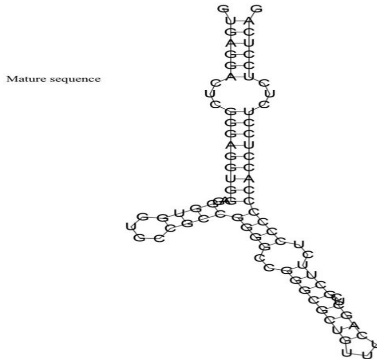
Figure 1. Secondary structure of has-miR-1224-5p.
