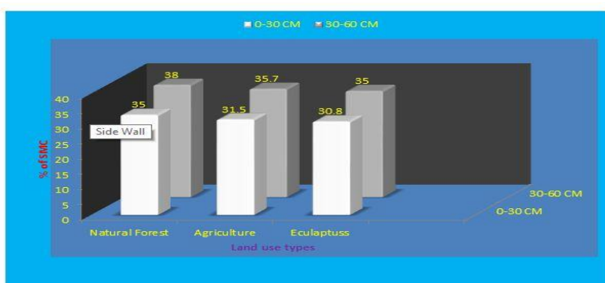
Figure 2. Soil moisture content affected by level soil bund at 0-30 and 30-60 cm.
