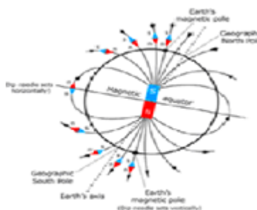
Figure 2. Close up depiction of the Earth's geomagnetic field lines.
