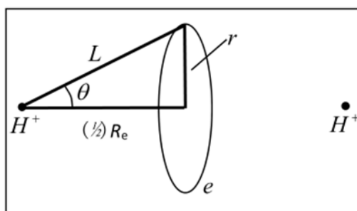
Figure 1. Hydrogen molecule-ion H_2^+ .
