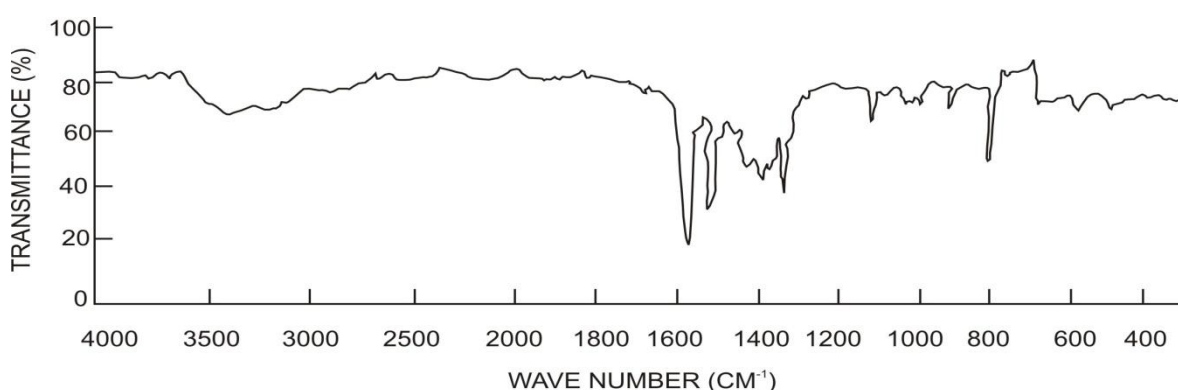
Fig. 1 : INFRARED SPECTRA OF Pt(NO 2 -acac) 2 in Carbon Tetra Chloride
