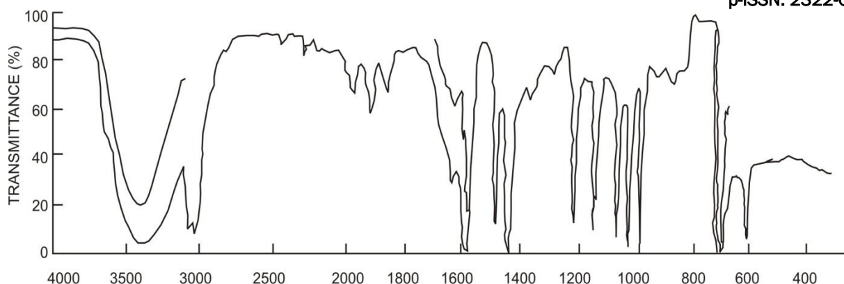
FIG. 2. INFRARED SPECTRA OF \text{Pt}(\text{NO}_2\text{-acac})_2 + PYRIDINE COMPLEX IN CARBON TETRA CHLORIDE
