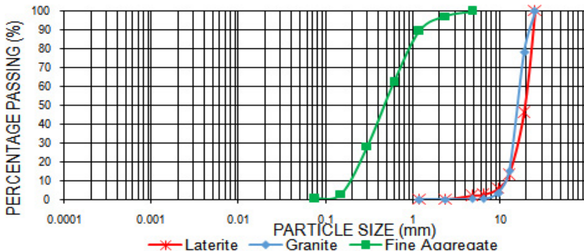
Figure 3. Particle size curves of lateritic nodules [6].
