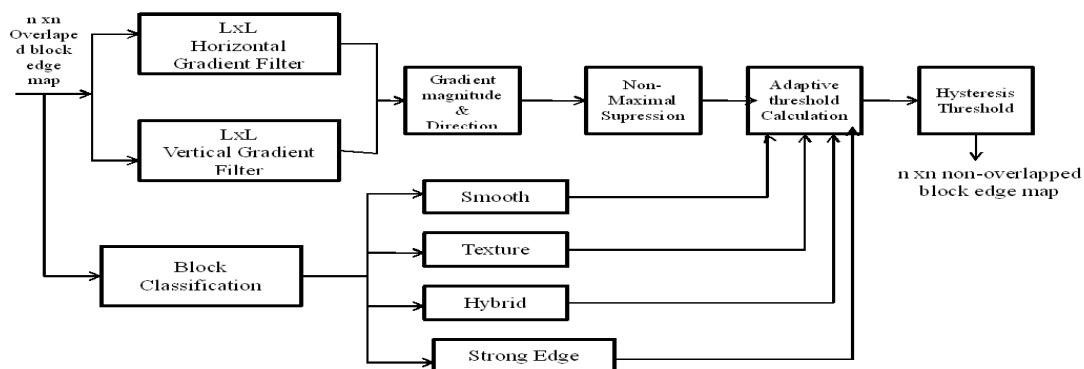
Fig.3: Distributed Canny Edge Detection Algorithm Block Diagram
