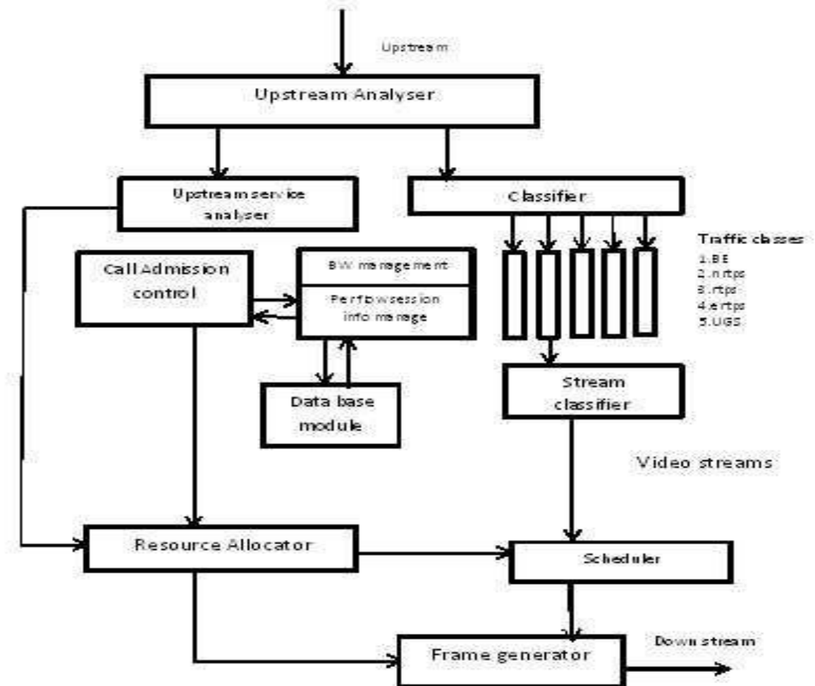
Figure 3. Frame Work model for video streaming Through WiMAX
