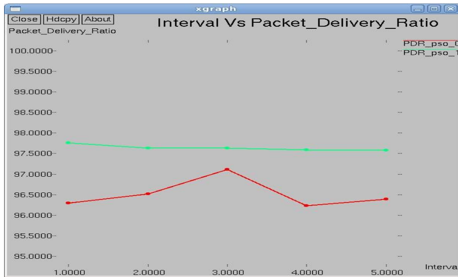
Figure.4 interval vs packet Delivery ratio with different kind of WiMAX traffic
