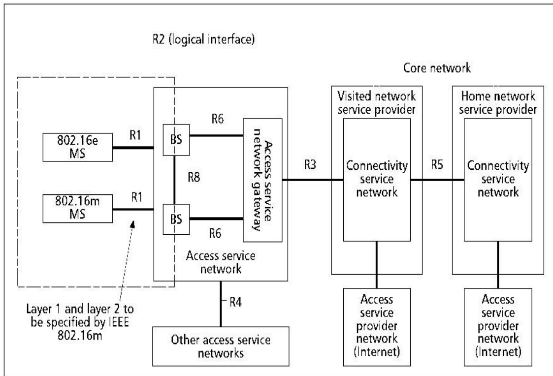
Figure.1 WiMAX Reference Model
