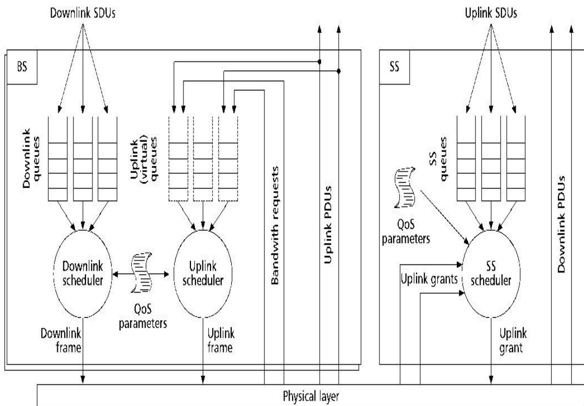
Figure.2 QoS tasks within BS and SS Architecture
