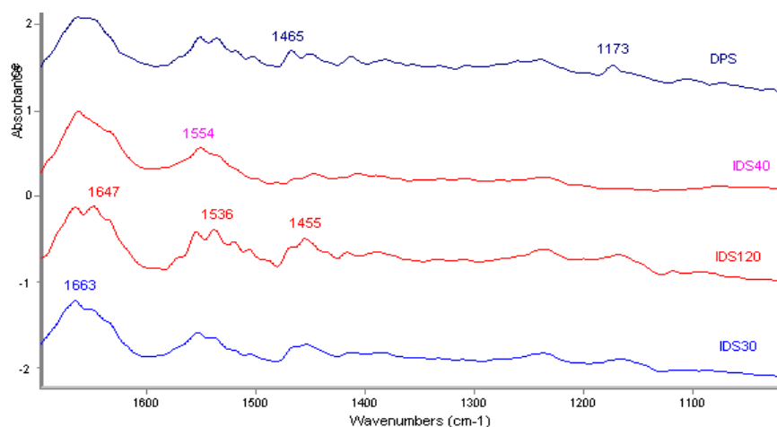
Figure 4. Fragment of FTIR spectra: dry pure chicken skin (DPS); dry chicken skin heated to boiling point for 30s and then incubated in presence of HSA at about boiling point for 30s (IDS30); dry chicken skin heated to boiling point for 40s and then incubated in presence of HSA at about boiling point for 40s (IDS40); dry chicken skin heated to boiling point for 120s and then incubated in presence of HSA at about boiling point for 120s (IDS120).
