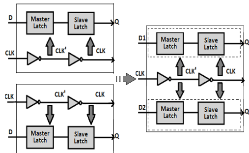
Figure 3: An example of merging two 1-bit flip-flops into one 2-bit flip-flop.
