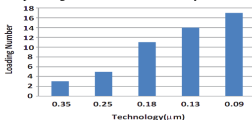
Fig. 1. Maximum loading number of a minimum-sized inverter of different technologies.
