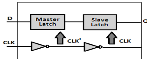
Figure 2: Single-Bit Flip-Flop
