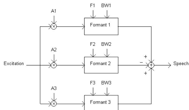
Fig. 3 Basic structure of a parallel formant synthesizer.
