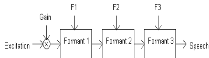
Fig. 2. Basic structure of cascade formant synthesizer.
