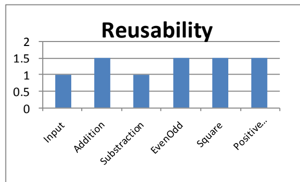
Graph 1: Maximum reusability
