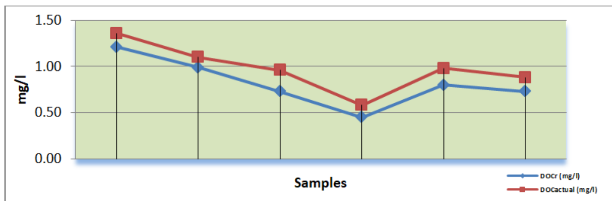
Figure 2. Dissolved organic matter prediction through river filtration.
