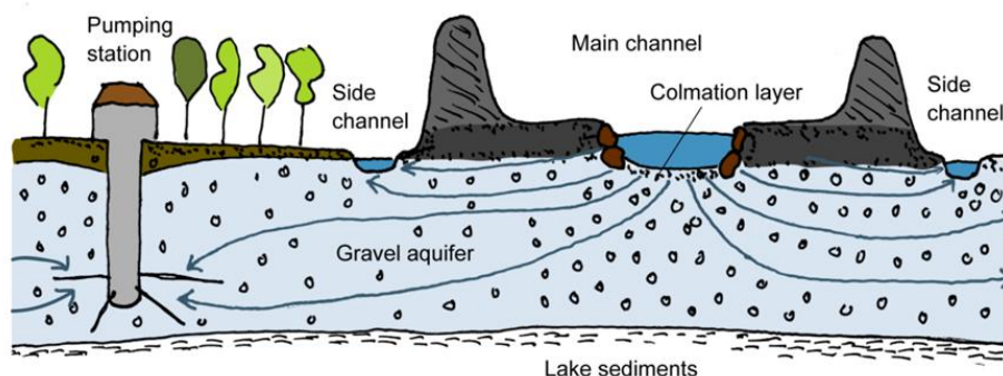
Figure 1. River bank filtration diagram.
