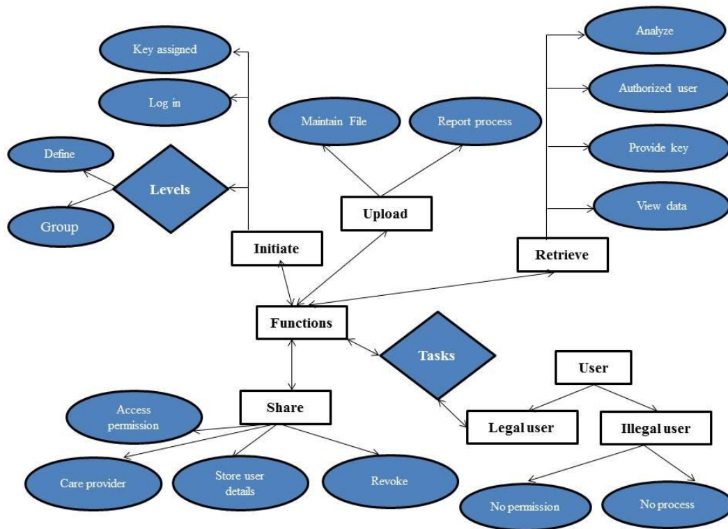
Fig 3. ER-Diagram For User Process
