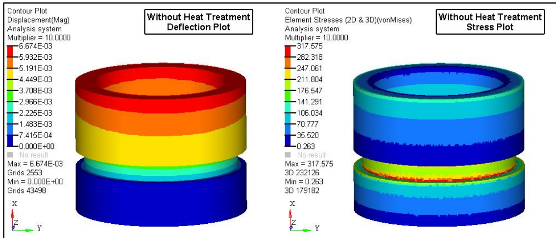
Fig7.: Deflection and Stress Plot (Cup without Heat Treatment)
