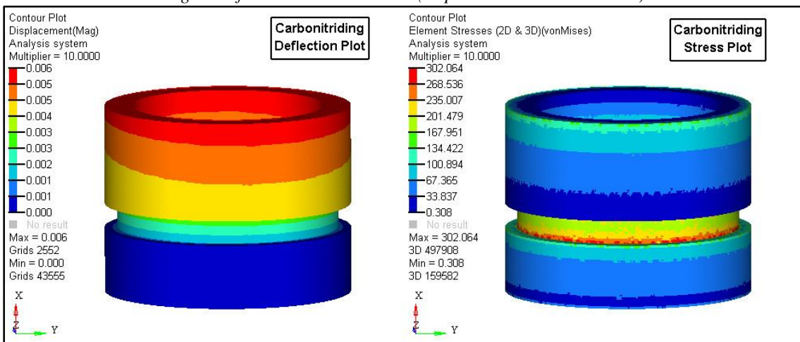
Fig8: Deflection and Stress Plot (Carbonitriding)
