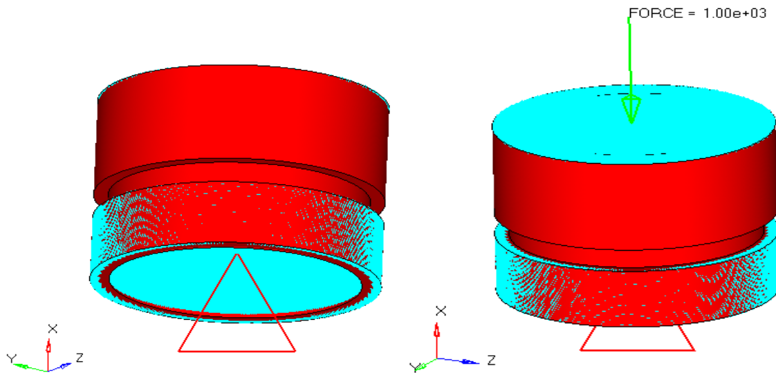
Fig.5: Boundary conditions applied on the bearing cup
