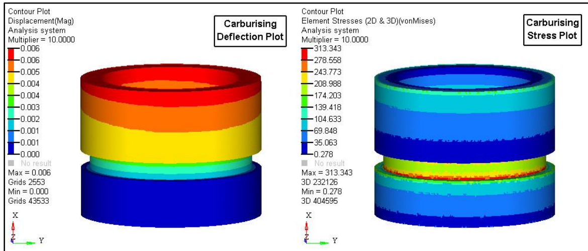
Fig.10: Deflection and Stress Plot (Carburising)
