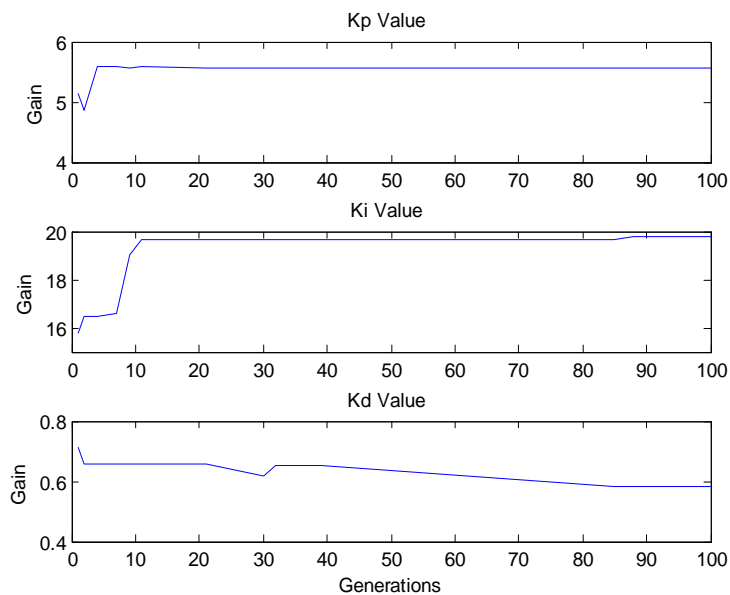
Fig 4: Iterations of all gain values
