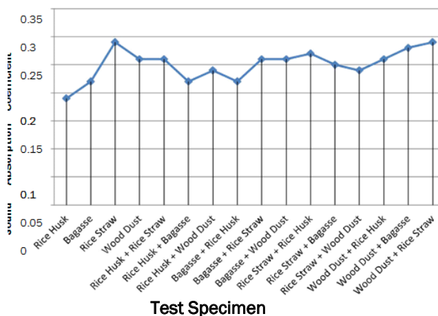
Figure 9. Sound absorption coefficient for rice straw and composition of rice straw and wood dust were maximum and around 0.29.
