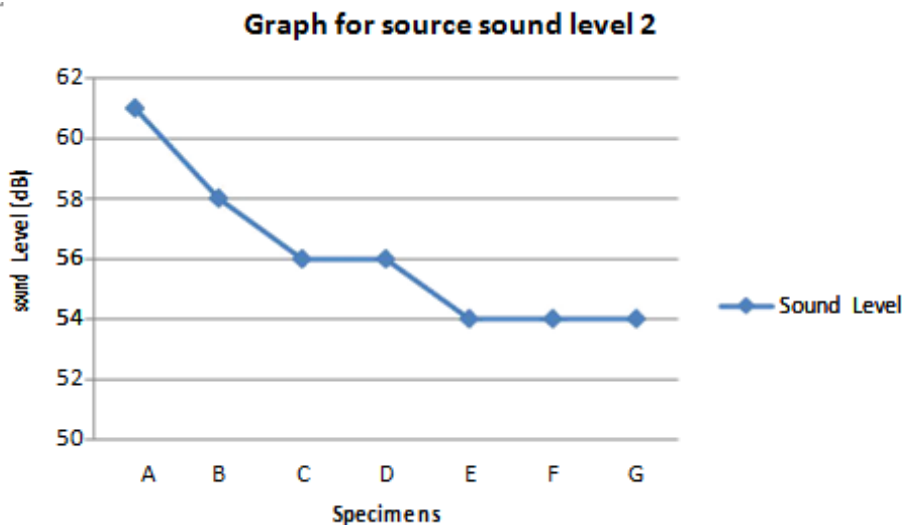
Figure 8. For source sound level 2 of 74 dB (40 mm thickness specimen in each case).
