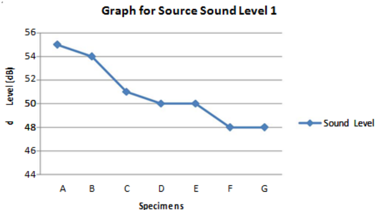
Figure 7. For source sound level 1 of 70 dB (40 mm thickness specimen in each case).
