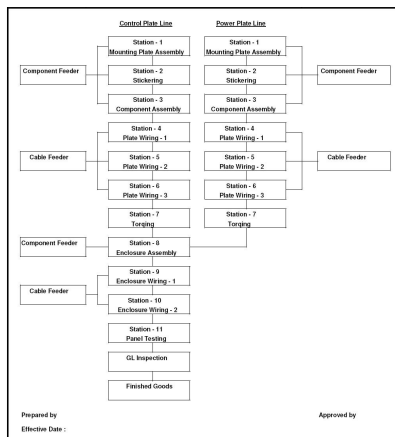
Fig-10 Modified Lay out
