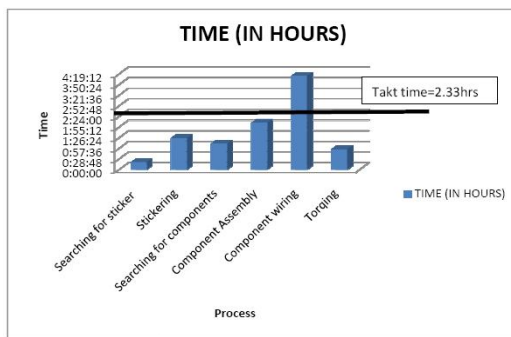
Fig-6 Electrical work- Power side
