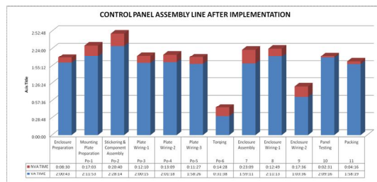
Fig-6.1 Line Balancing After Implementation
