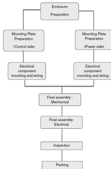
Fig.1 process flow
