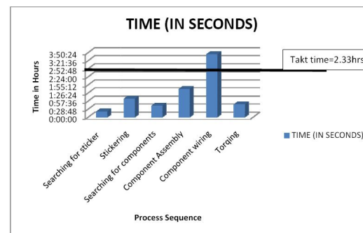
Fig-4 Electrical work- Control side
