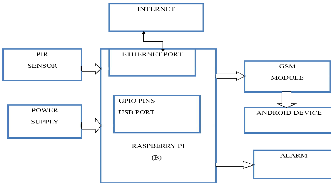
Figure 1: Hardware component of the proposed project.
