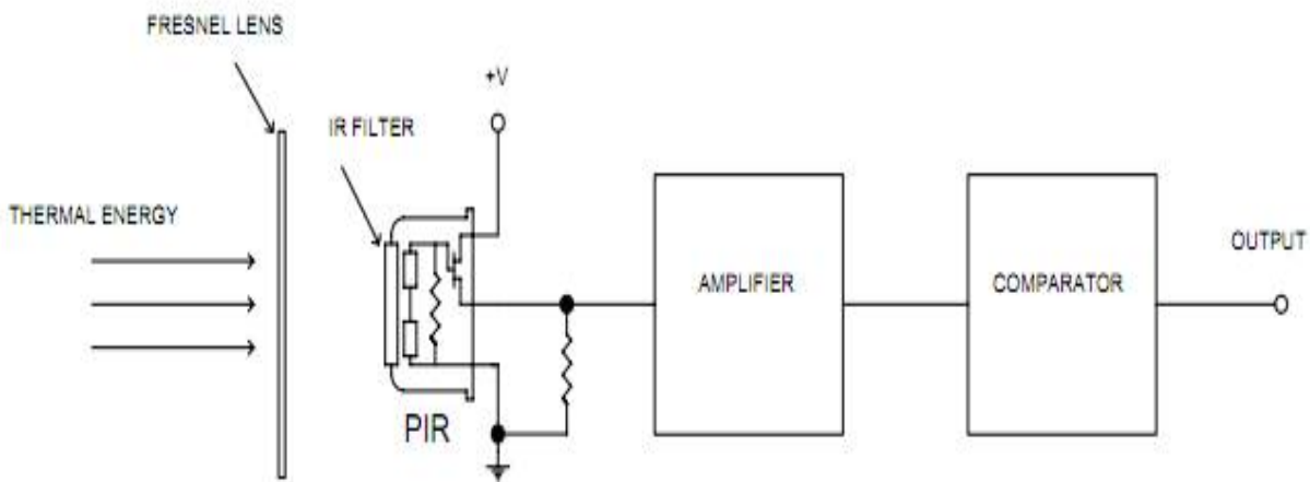
Figure 2: Typical configuration of PIR sensor.
