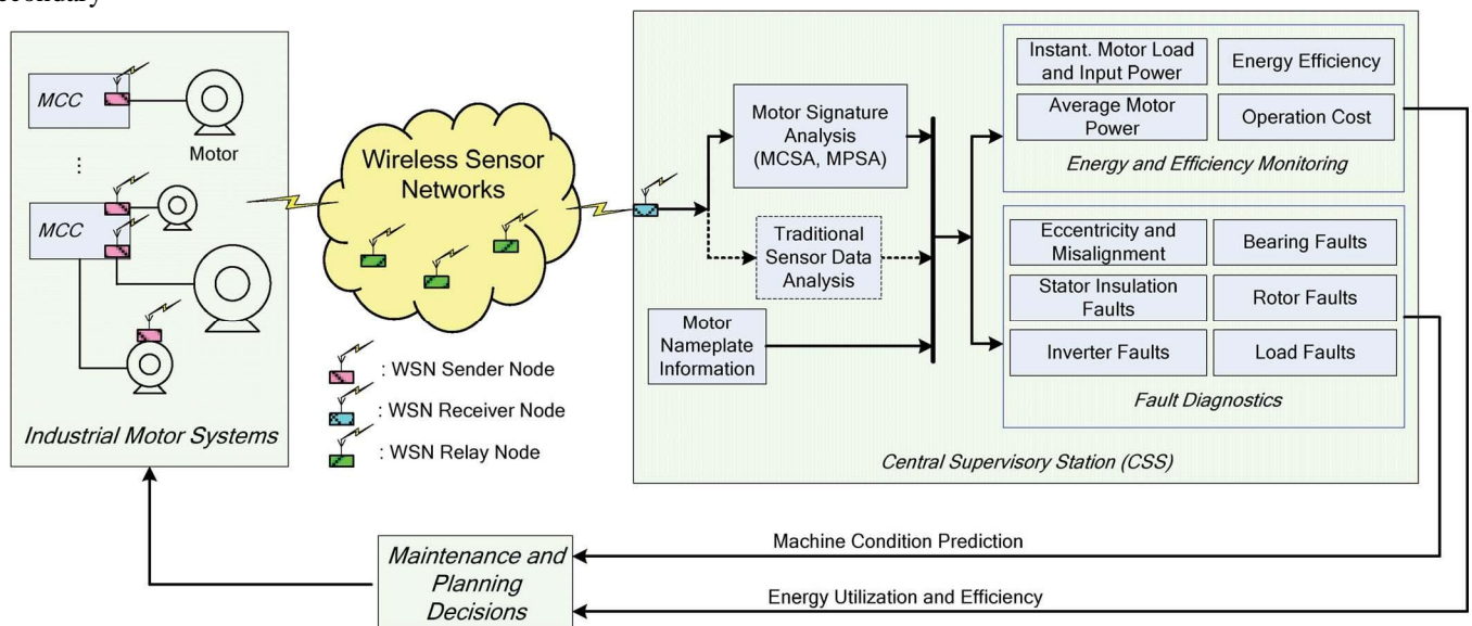
Fig. 1. Online and remote energy monitoring and fault diagnostics for industrial motor systems using WSNs.
