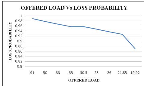
Fig 4. Per node loss probability versus the offered load .
