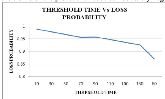
Fig 6. MAC layer loss probability versus the average threshold waiting time
