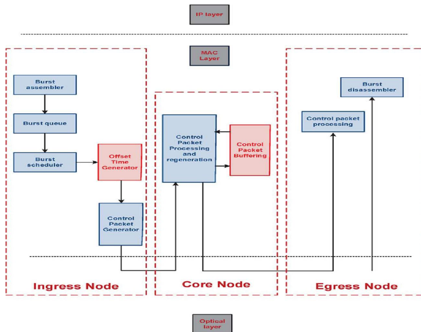
Fig. 3. OBS MAC layer with the proposed CP buffering feature.
