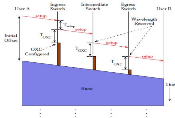
Fig 2. Immediate wavelength reservation
