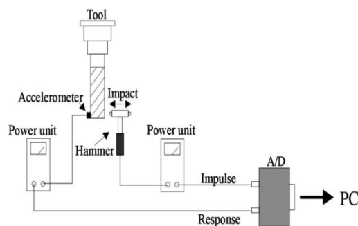
Figure 4. Measurement of the impulse response
