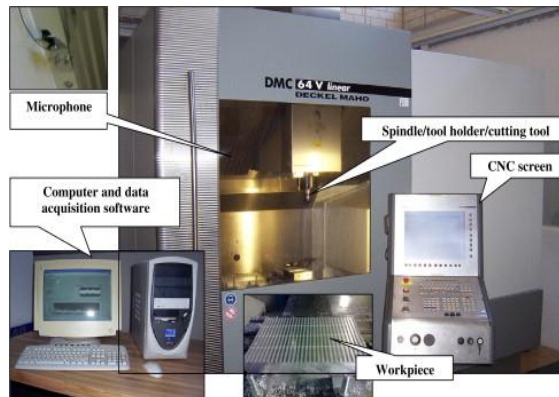
Figure 2. Experimental setup for finding stability lobe diagram.[11]
