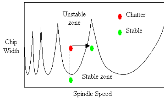
Figure 1. Example of a stability lobe diagram (SLD) and the stable and unstable cutting conditions
