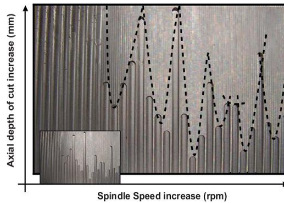
Figure 3. SLD marked on workpiece surface.
