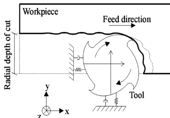
Figure 6. Dynamic milling force model.
