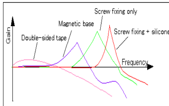
Figure 5. Frequency characteristics on sensor fixing ways
