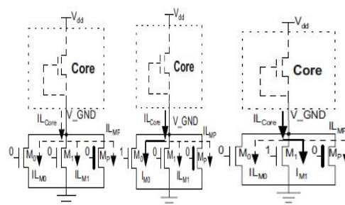
Figure: 1 Multi-Mode power gating Architectures: a) Snore mode b) Dream mode c) Sleep mode
