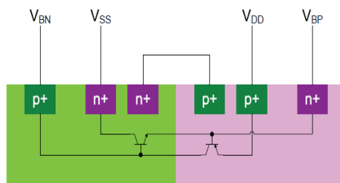
Figure 3: Leakage path in forward body biasing
