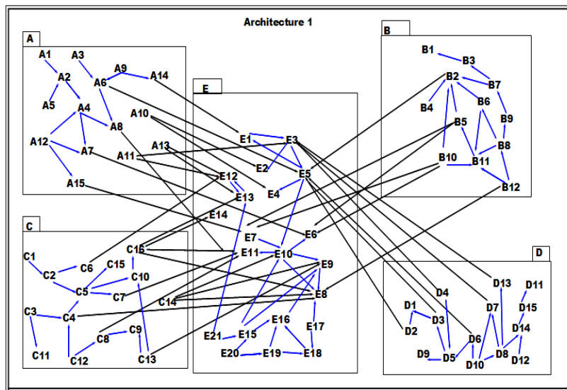
Fig. 1 An initial architecture composed of classes and packages.
