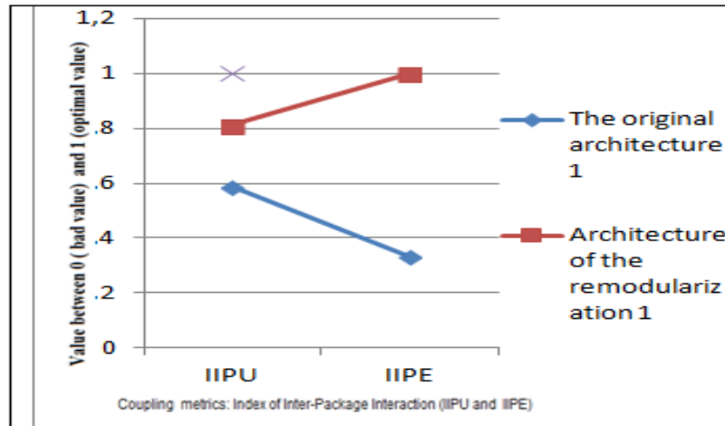
Fig. 6 Graphic representation of Coupling metrics: Index of Inter-Package IIPU and IIFE (table2).
