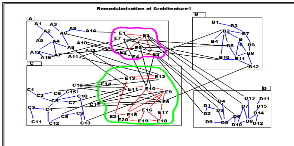
Fig. 4 One possibility of remodularization
