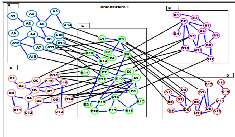
Fig. 2 Original architecture of Figure 1 as nodes relative to classes and arcs relative to the relationship between these classes.
