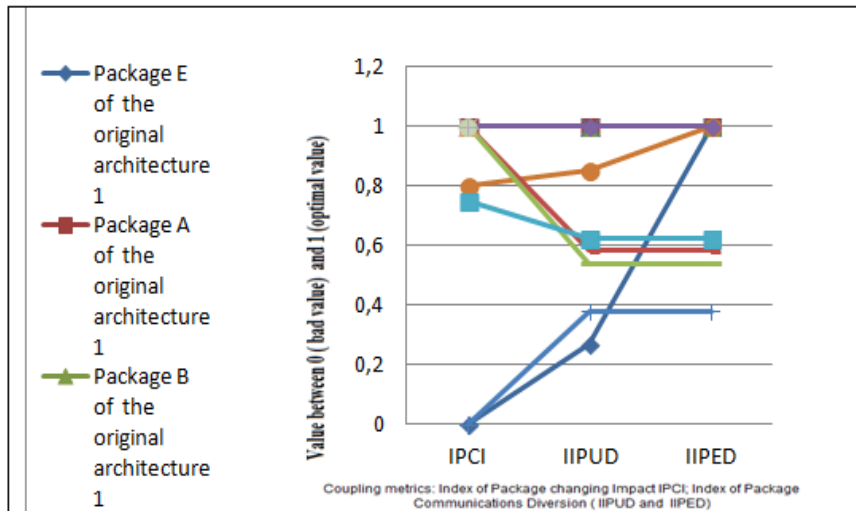
Fig. 7 Graphic representation of Coupling metrics: Index of Package changing Impact; Index of Package Communications Diversion (table3).
