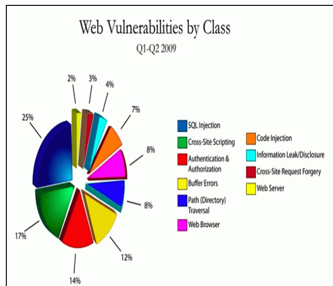
Figure 1 - Web Vulnerabilities
